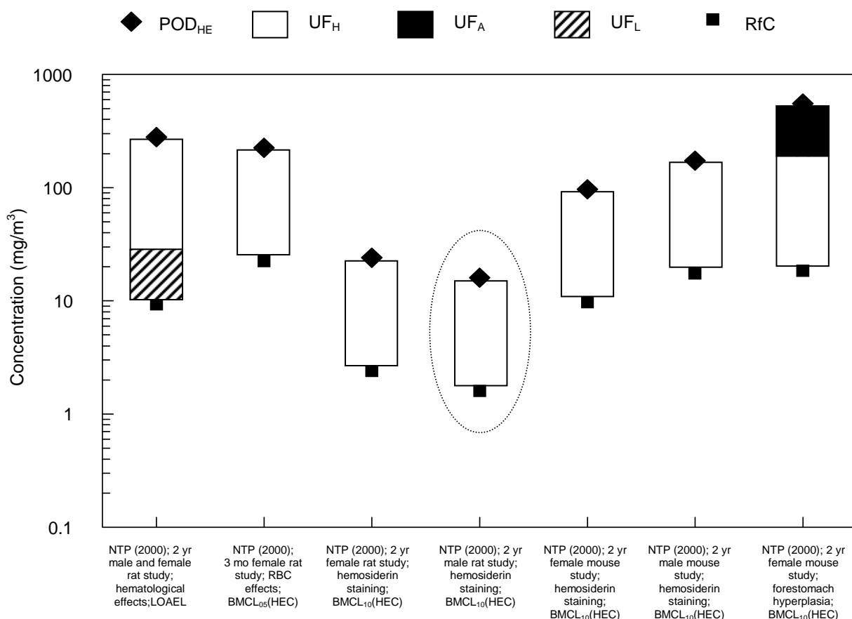
Figure 5-1. PODs for selected endpoints with corresponding applied UFs and derived RfC.
